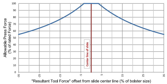
Permissible eccentric load (Mechanical Press)
